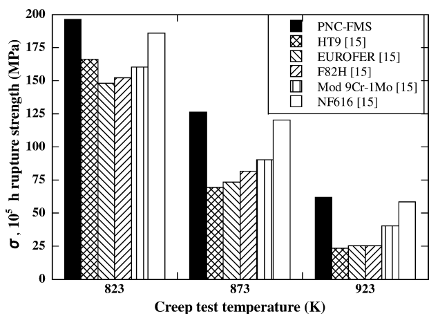
Fig. 2. Comparison of the 10 5 h rupture strengths for PNC-FMS, Sandvik HT-9, EUROFER, F82H, modified 9Cr-1Mo and NF616 at 823, 873 and 923 K.
