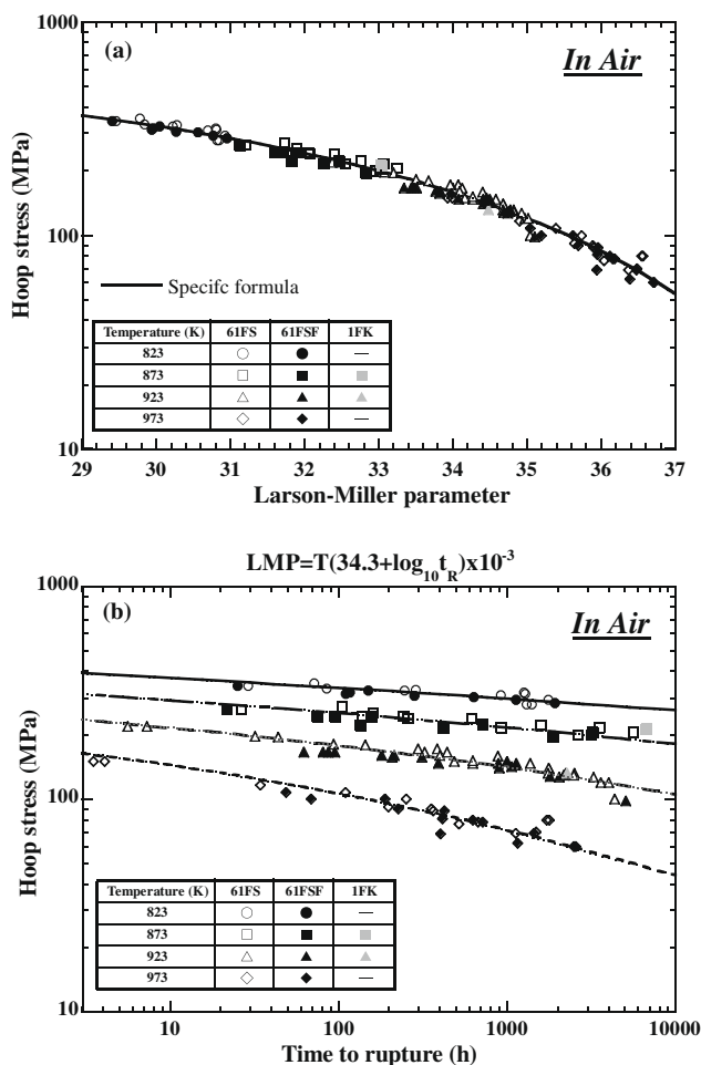
Fig. 1. Summary of the thermal stress rupture behavior of as-received PNC-FMS cladding. (a) The rupture time t_R is in hours and the temperature T is in Kelvin in the Larson-Miller parameter. (b) Relationship between hoop stress and time to rupture at the temperature from 823 to 973 K. The trend curve indicates the fitting from LMP.
