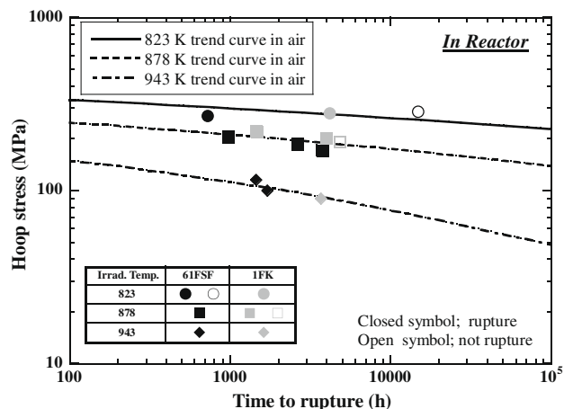
Fig. 3. Results of in-reactor creep rupture tests of PNC-FMS at temperatures of 823, 878 and 943 K.
