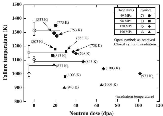
Fig. 5. Relationship between transient burst strength and neutron dose of irradiated PNC-FMS claddings. Error bars with maximum and minimum data points are for as-received specimens.
