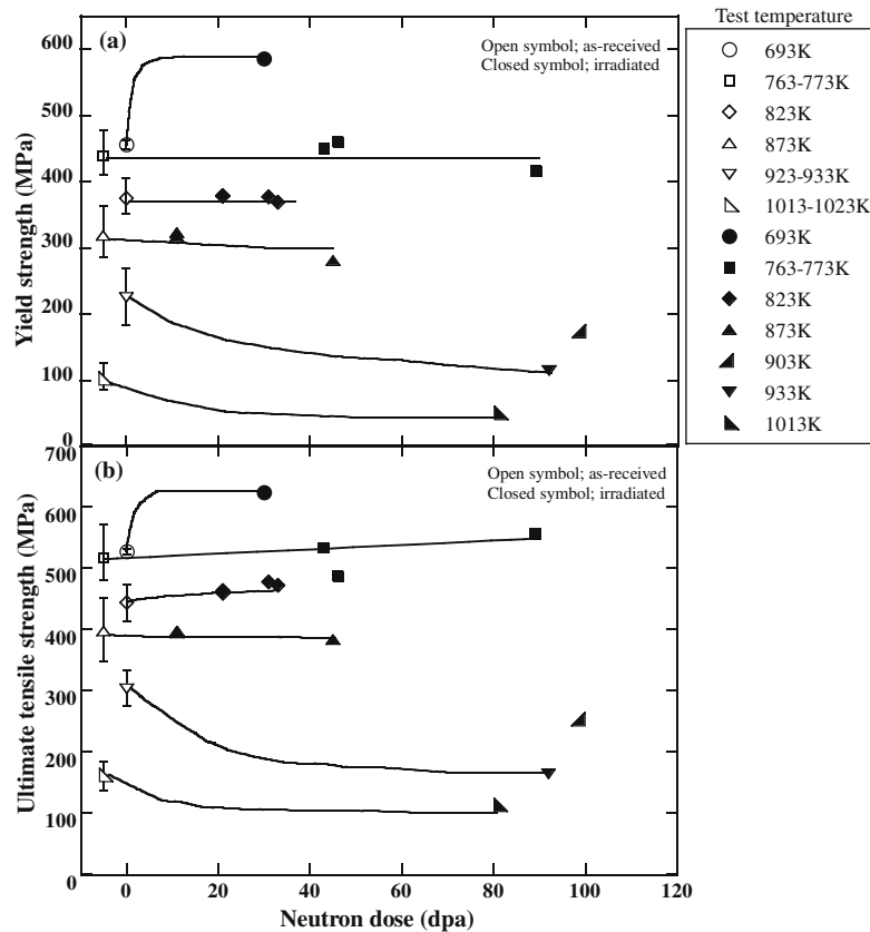
Fig. 4. Relationship between tensile strength and neutron dose of irradiated PNC-FMS claddings: (a) yield strength and (b) ultimate tensile strength.
